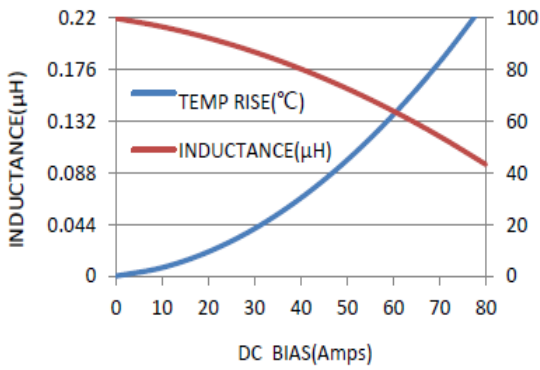
MCMB-1340-R68MT
