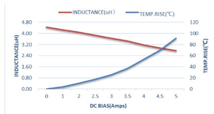
MTQH322520S4R7MBT
