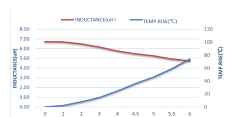
MTQH404030S6R8MBT
