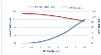
MTQH404020S150MBT
