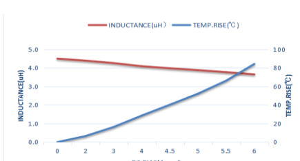
MTQH404030S4R7MBT
